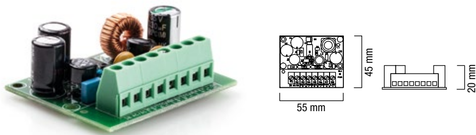
V 4512 16 - 24 Vdc or 17 - 32 Vac voltage reducer with internal stabilizer and signaling LED of reducer activated. Output: 12 - 13.8 Vdc.
