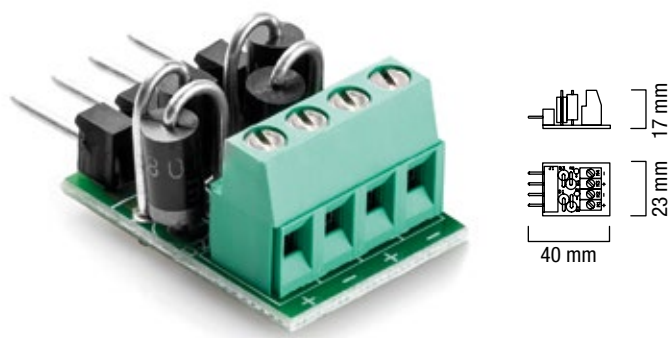
V 12 Voltage reducer from 13.8 Vdc to 12 Vdc for infrared TV cameras and other products. 2 outputs of max 1 Ah each.
